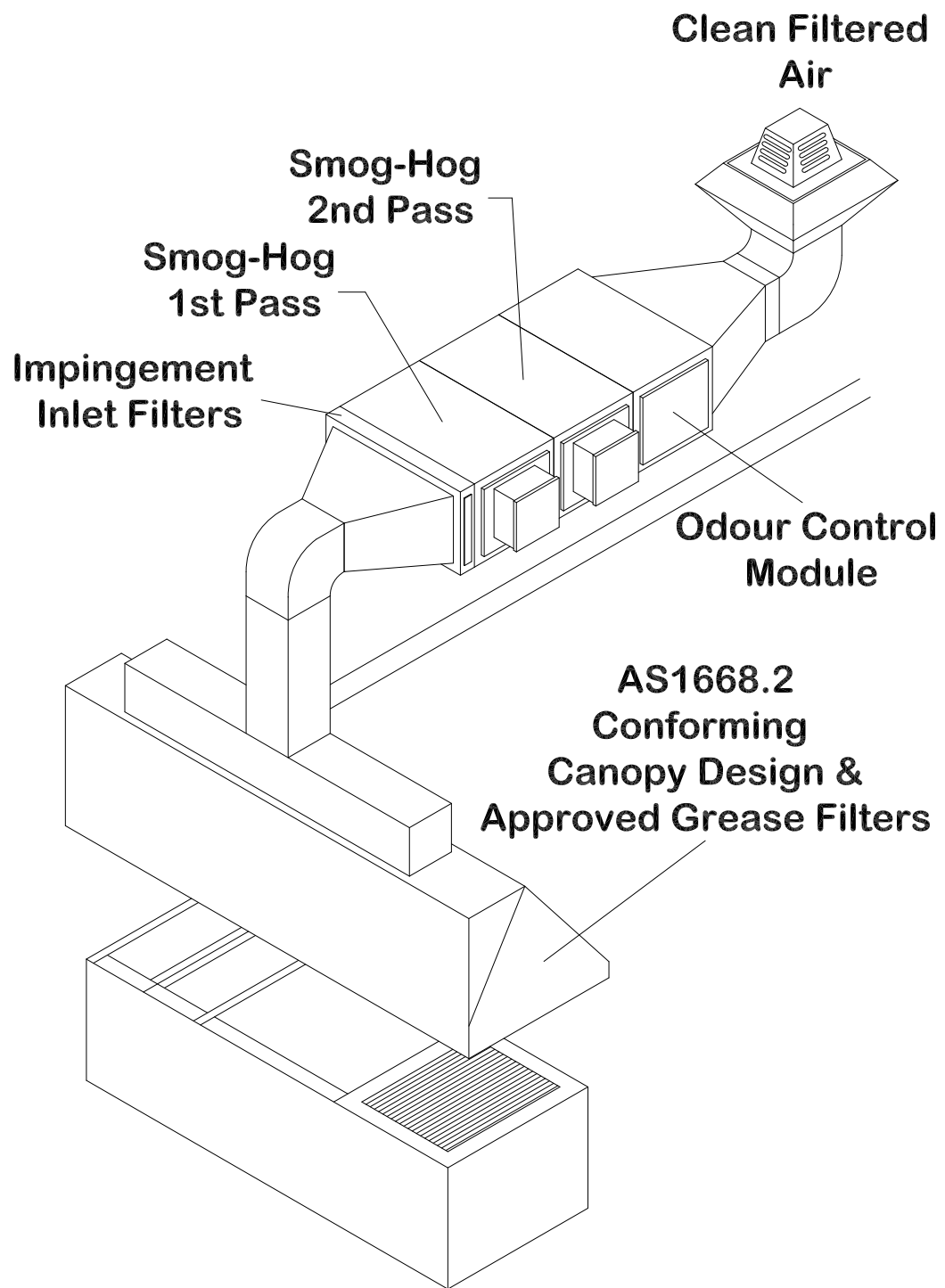
Typical Smog-Hog Roof Mounted Installation
