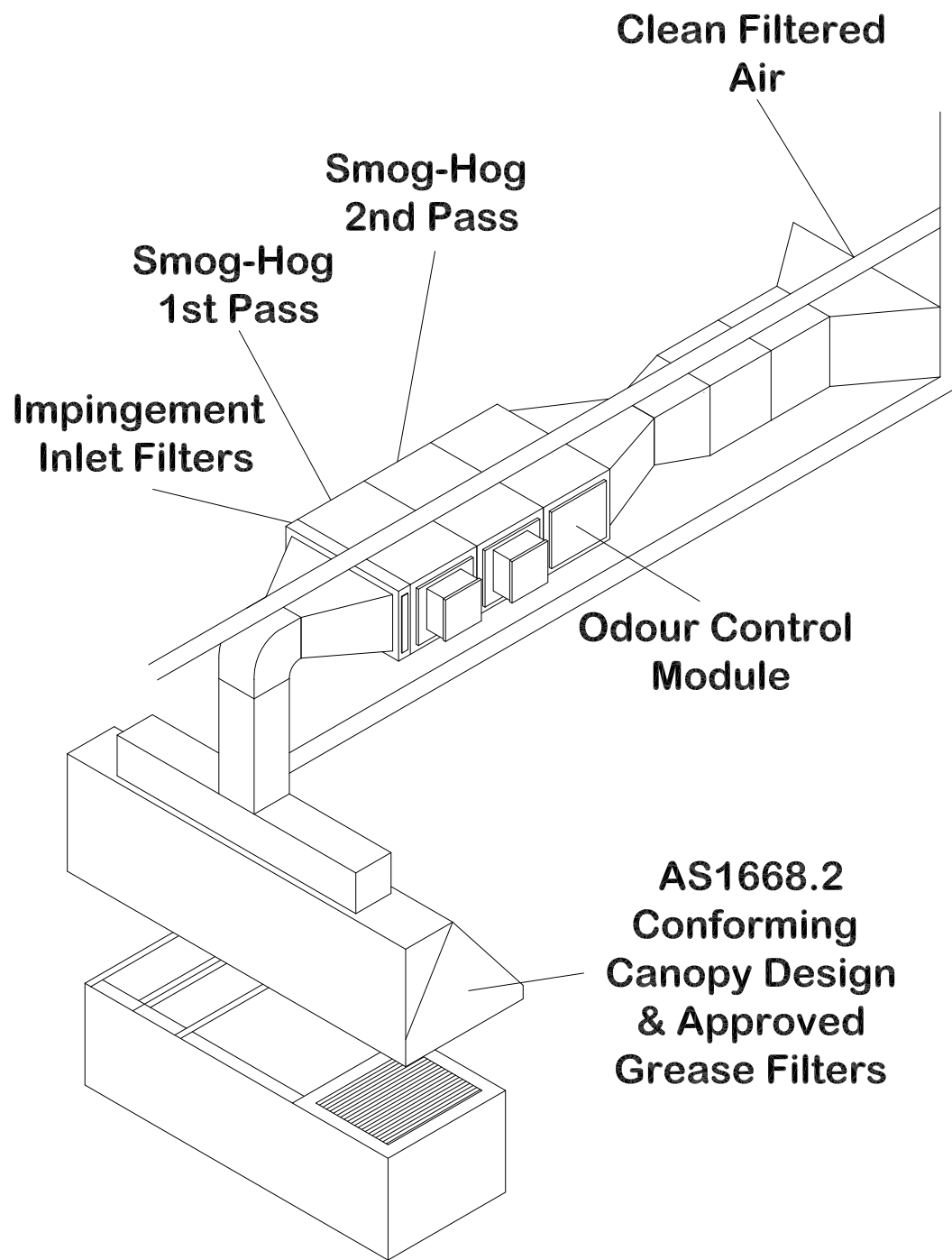
Typical Smog-Hog Low Level Horizontal Discharge Installation
